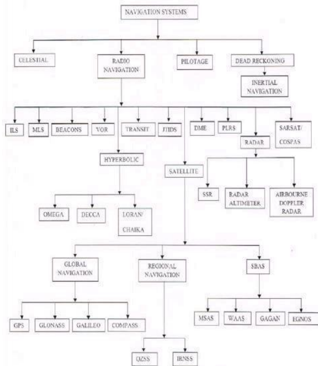
Fig:1 The classification of modern navigation system
