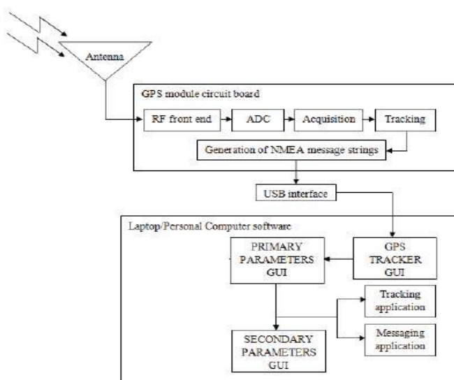
Fig.4 shows GPS receiver system block diagram
