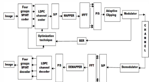
Fig. 2: The modified OFDM system diagram
