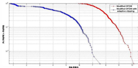
Fig. 6: CCDF comparison of PAPR for the modified OFDM system with and without adaptive clipping over AWGN channel with QAM16 mapping
