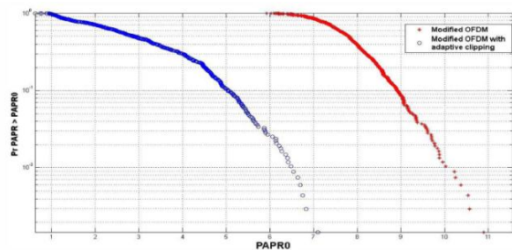
Fig. 4: CCDF comparison of PAPR for the modified OFDM system with and without adaptive clipping over AWGN with QPSK mapping
