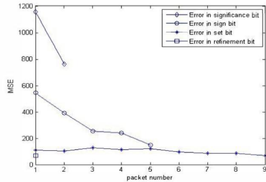
Fig. 1: Error bit sensitivities within the SP IHT coded bit stream
