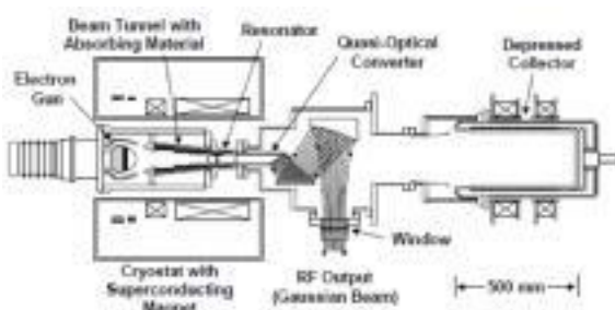
Fig. 1. Typical Gyrotron [1]
