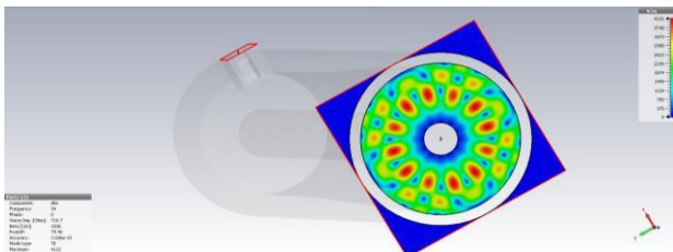
Fig.6. Mode Pattern Of TE 62 mode
