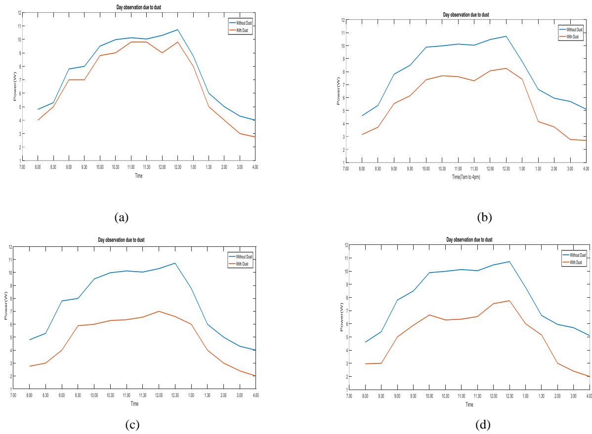
Fig 2: Periodically measured output power vs time for two solar panels, one without dust (blue) and another with dust (red), (a) after 5 days (b) after 1 week (c) after two weeks and (d) after three weeks.
