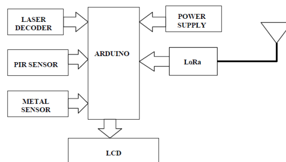
Fig. 1. Transmitter Node
