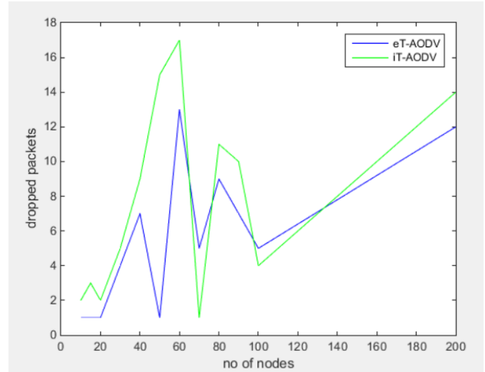
Fig 3: COMPARISON BETWEEN NO OF NODES AND DROPPED PACKETS
